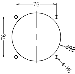
Installation cut out size
