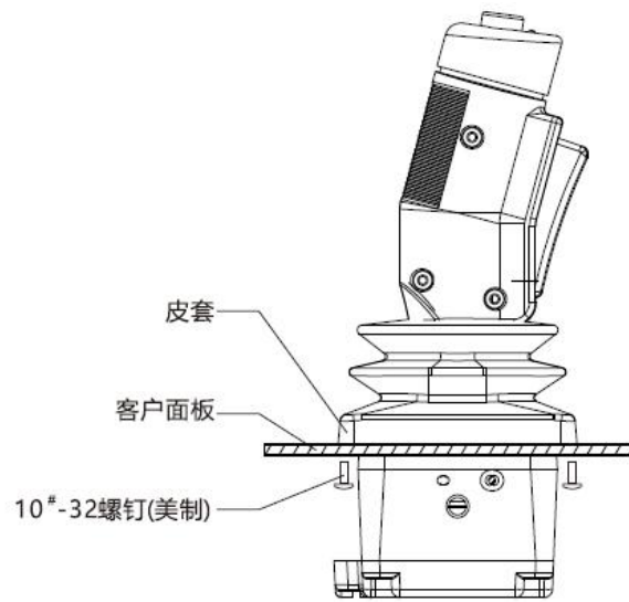
MOUNTING
